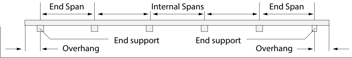
Span Definitions
